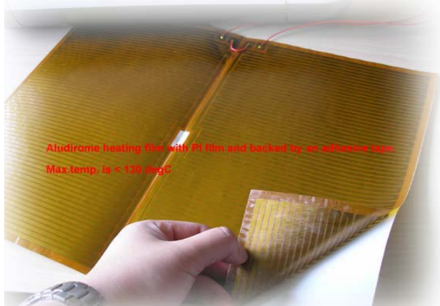
Aludirome heating film with PI film and backed an adhesive tape
